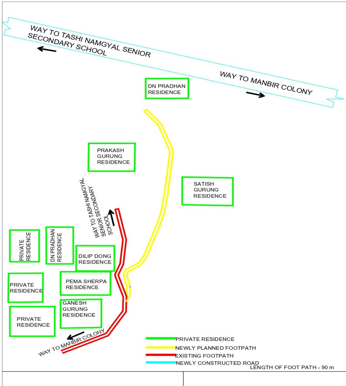
CONSTRUCTION OF FOOTPATH AT MANBIR COLONY
